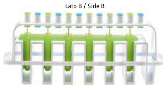
Green mould / Stampo verde Assembly / Assemblaggio
